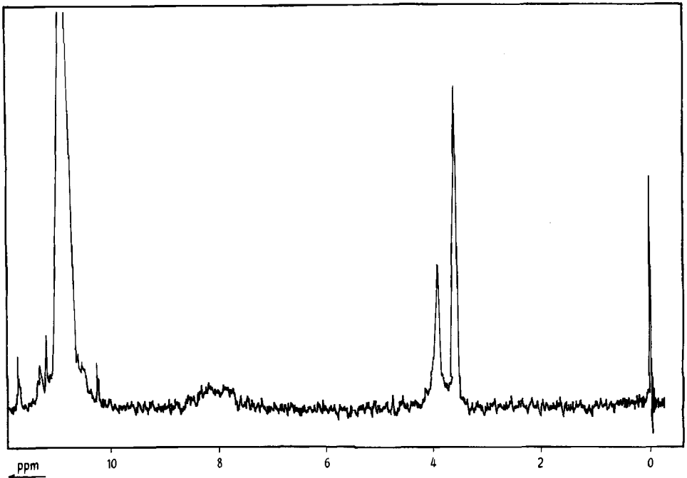
Fig. 6. NMR.-Spektrum von ( N -3)-Methyl-tetrahydropterin in CF_3COOH ( \delta_{TMS} = 0 ppm)
